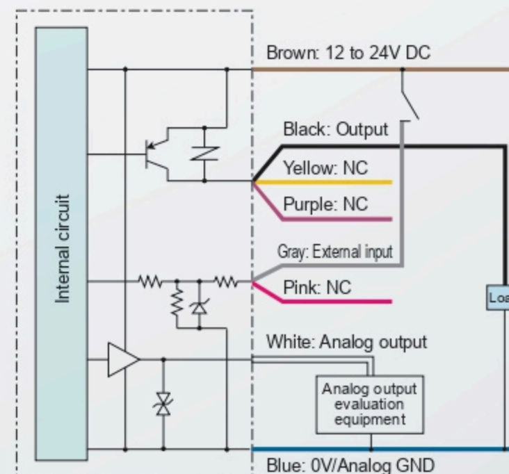
With the PNP setting
