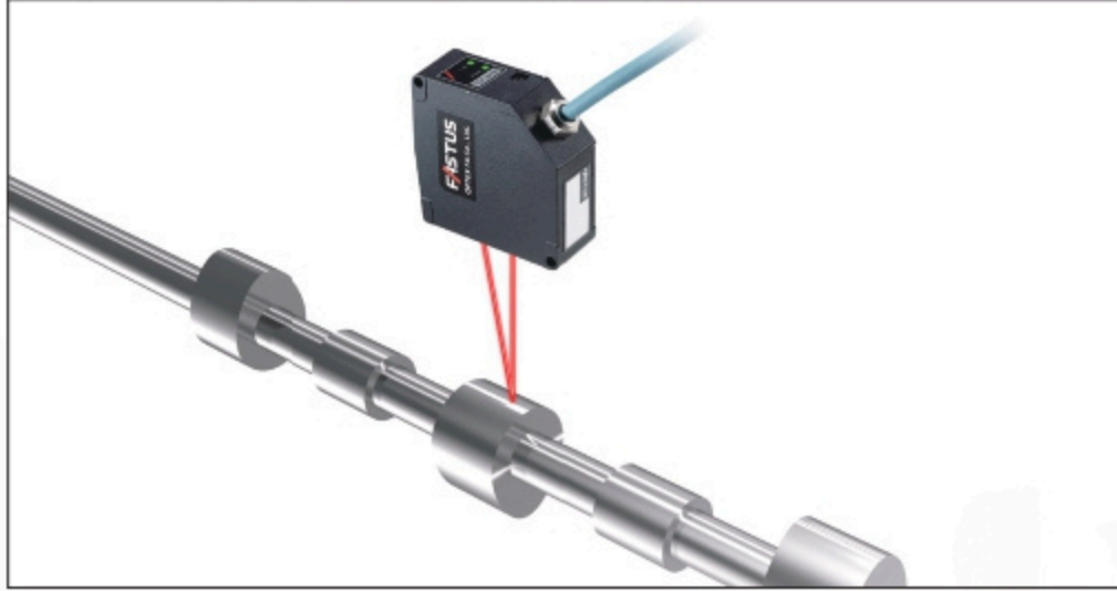
Shape measurement of cam shafts
