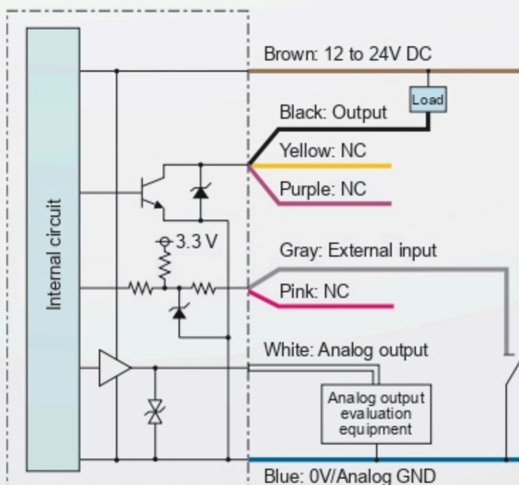
With the NPN setting
