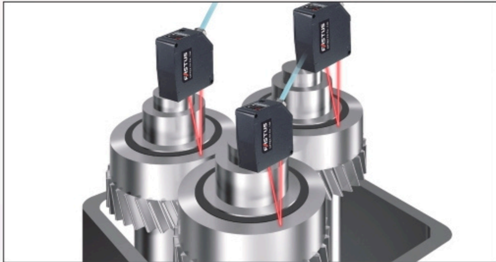
Flatness measurement of transmission parts
